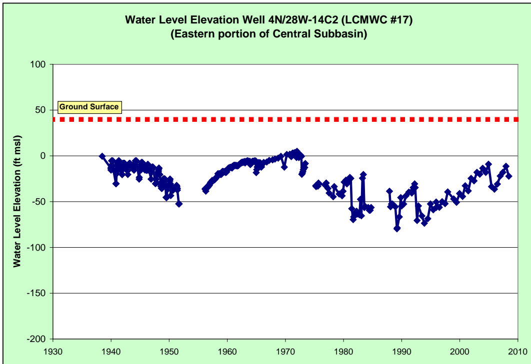
Figure 2-5. Hydrograph of well 14C2 in the eastern portion of the Central subbasin.
